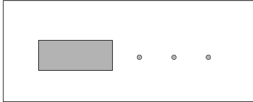
Front Panel Cutout Template LED Holes = 1/4"
