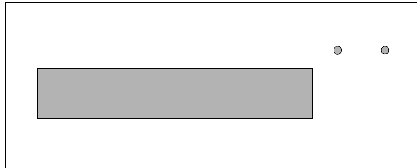
Back Panel Cutout Template MOSFET Mounting Hole Size = 1/8"
